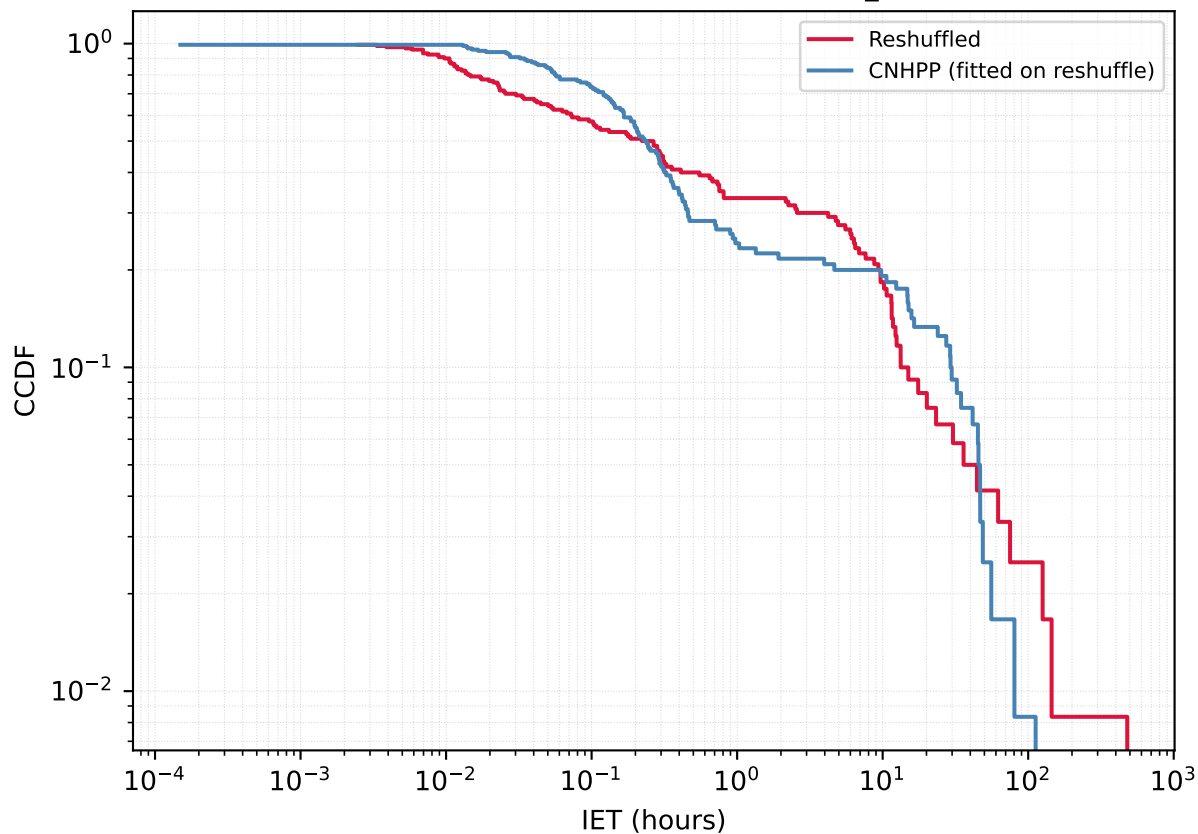
User 1131058651 - Reshuffled vs CNHPP A_{\text{fit}}=0.9261
